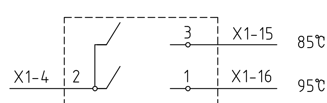
LIQUID TEMPERATURE INDICATOR 1
