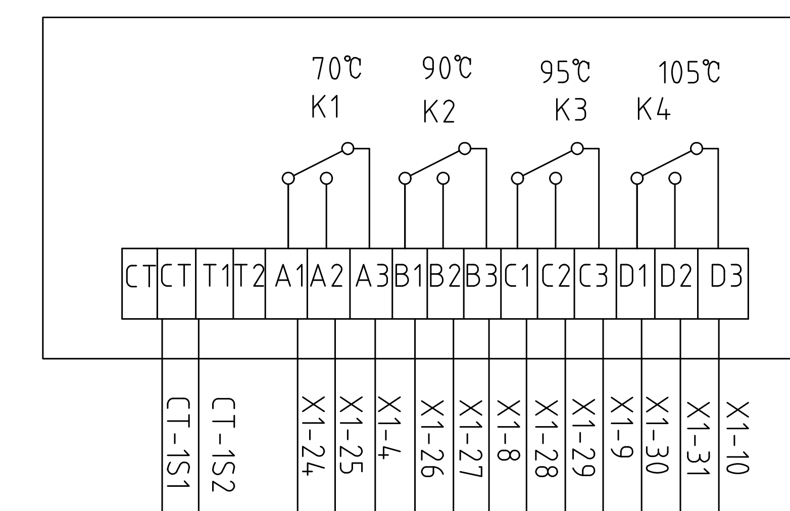
Winding thermometerBWR-4
